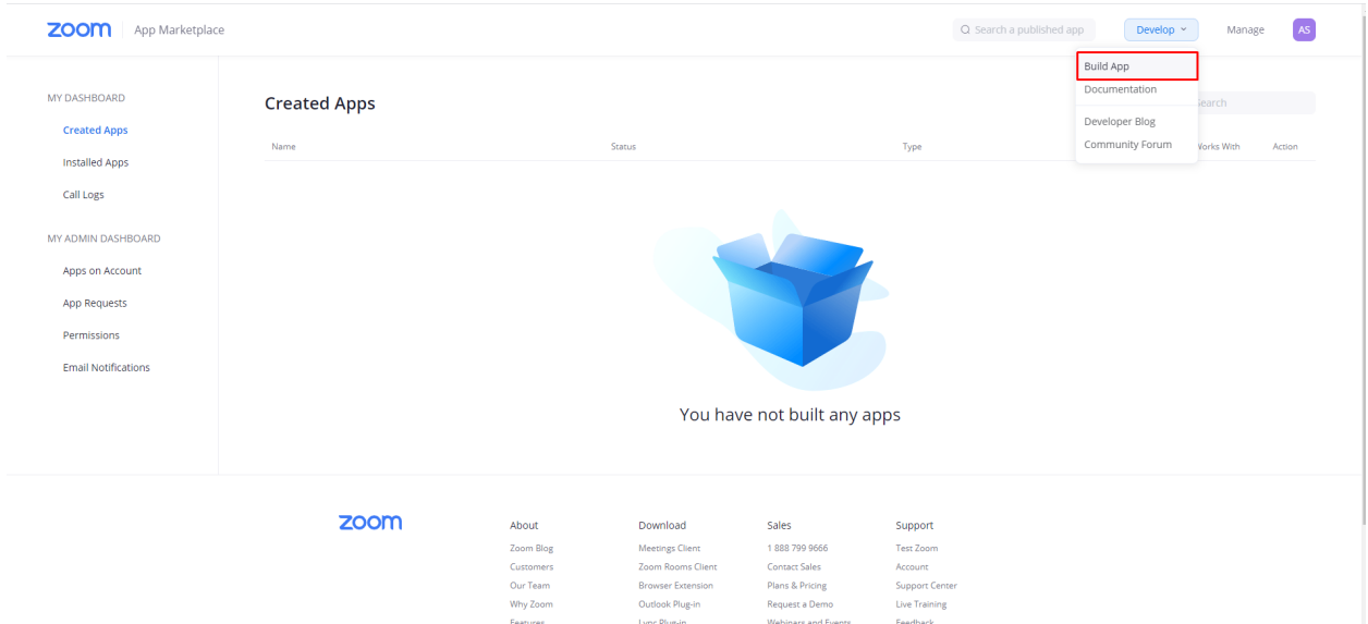
Fig. 3: Build App
