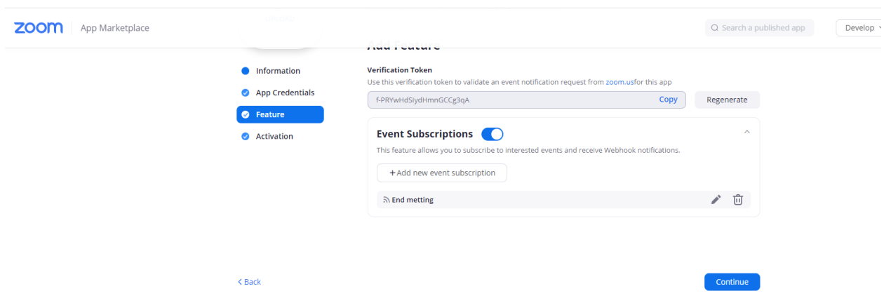
Fig. 10: Events added
