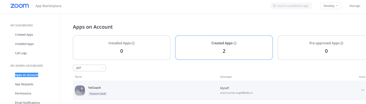
Fig. 12: App Listing
