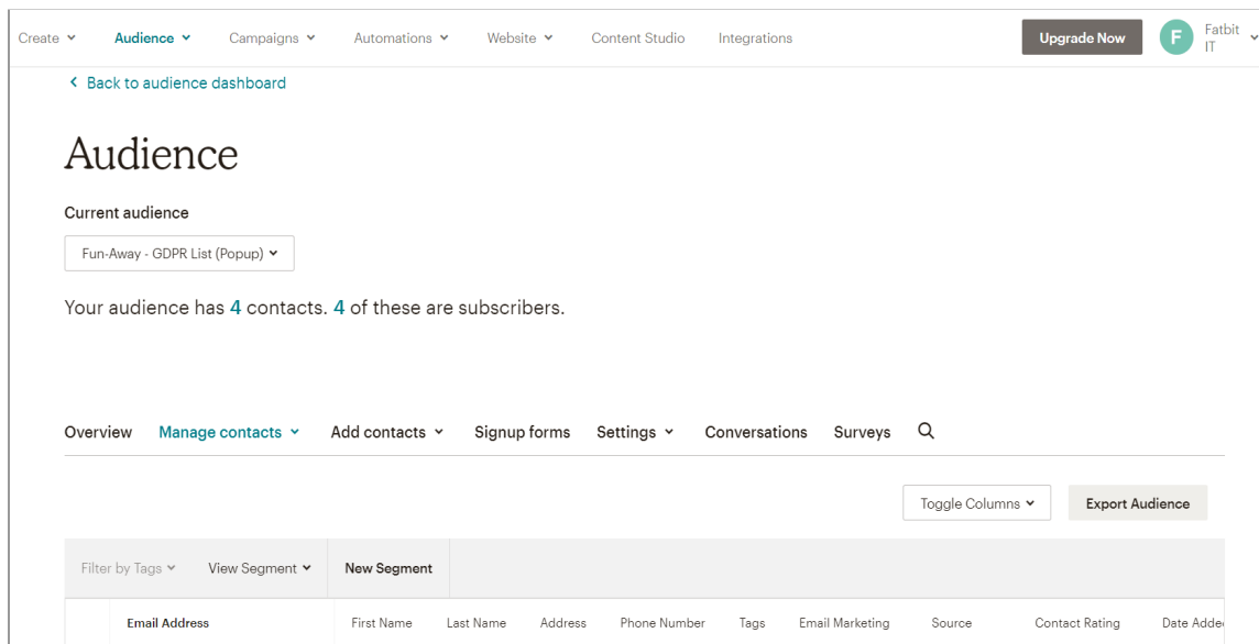
Fig. 6: 'Audience' Page
